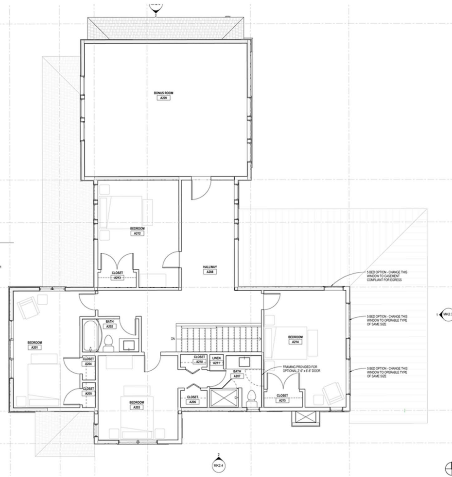
1 MAIN FLOOR PLAN - MKTG SCALE: 1/4" = 1'-0"
